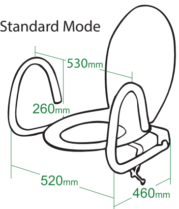
Splayed Mode
